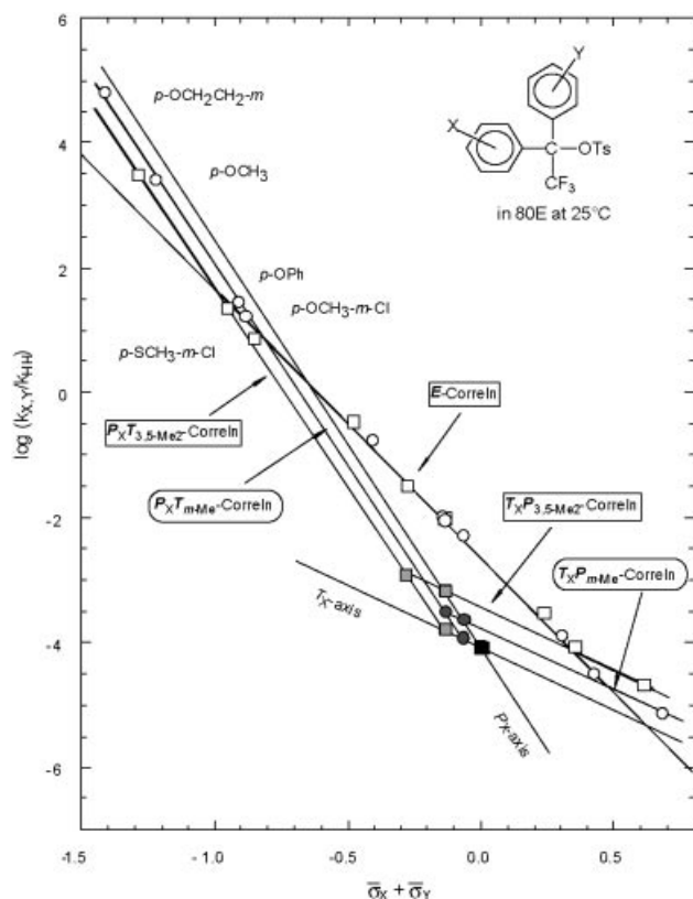
Figure 3. The Y-T plot for the solvolyses of 1-aryl-1-( m -methylphenyl)-2,2,2-trifluoroethyl tosylates ( 6 ) and 1-aryl-1-(3,5-dimethylphenyl)-2,2,2-trifluoroethyl tosylates ( 6a ). Open circles are for 6 , open squares for 6a , and closed symbols for lim PT-conformation (see text)
