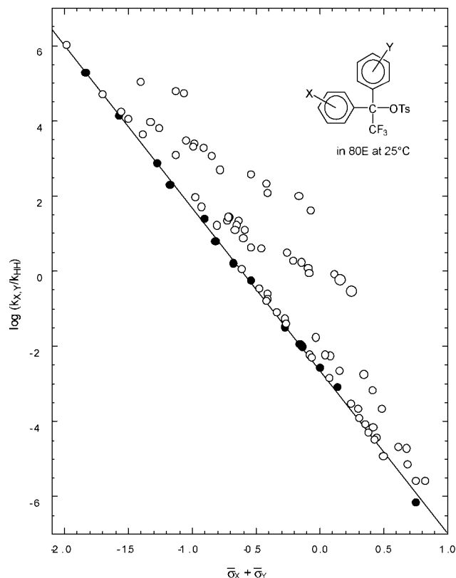
Figure 1. Additivity relationship against the sum of \bar{\sigma} ( r = 1.17 ) for substituent effects on the solvolysis of 1,1-diaryl-2,2,2-trifluoroethyl tosylates in 80% aqueous ethanol at 25 °C. Closed circles are for the symmetrical X = Y subseries 1
