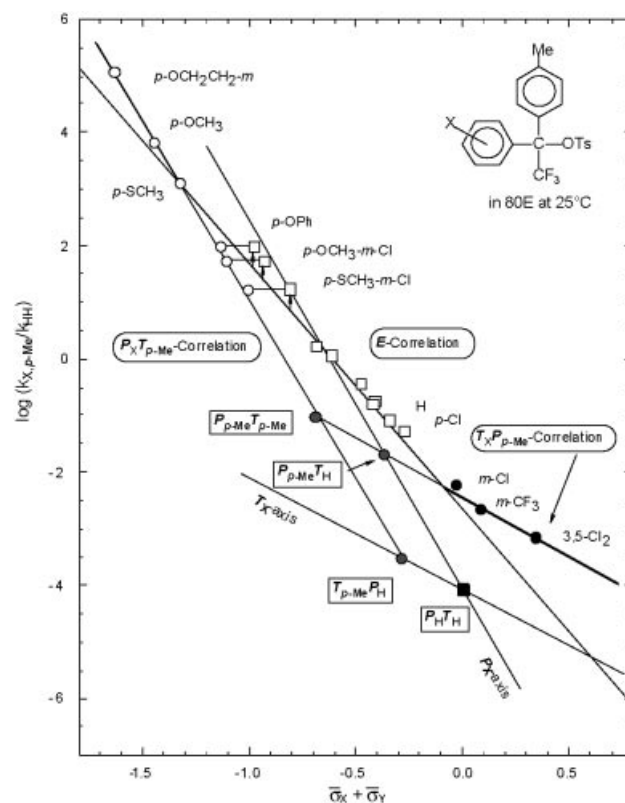
Figure 4. The Y-T plots for the solvolyses of 1-aryl-1-( p -methylphenyl)-2,2,2-trifluoroethyl tosylate ( 4 ). Open circles are for the P_X -conformer correlation against \bar{\sigma}_P ( r = 1.505 ), open squares are for the E -conformer correlation against \bar{\sigma}_E ( r = 1.17 ) and closed circles are for the lim T_X correlation against \bar{\sigma}_T ( = \sigma^0 )
