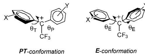
Scheme 1. Coplanarity change in 1,1-diaryl-2,2,2-trifluoroethyl cation. E conformation : equivalent propeller conformation ( 23 < \theta_E < 38^\circ ); PT conformation : single aryl twisted conformation ( \theta_P = 9\text{--}15^\circ , \theta_T > 45^\circ )
