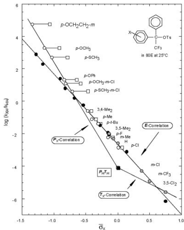
Figure 2. The Y–T plot for the solvolysis of 1-phenyl-1-(substituted phenyl)-2,2,2-trifluoroethyl tosylates ( 2 ). Open squares for the E -conformer correlation against \bar{\sigma}_E with r=1.17 , open circles for the P_X -conformer correlation against \bar{\sigma}_P with r=1.505 , gray circles for m -substituents against \sigma^0 and black circles for symmetrically disubstituted substrates defining the E -conformer correlation
